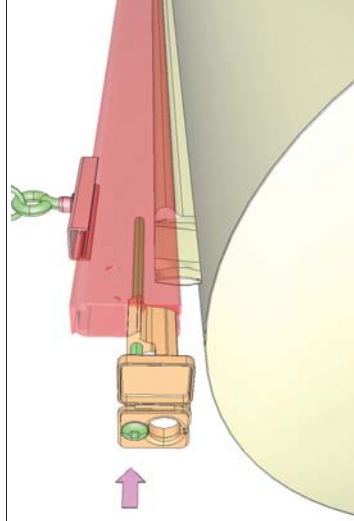
14. Put plastic end cap plug in place and have tensioner grab tensioning fabric pocket.
