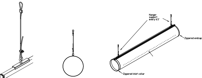
Fabric duct Installation Details Single Track Profile
