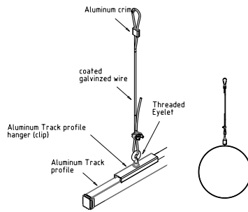
Fabric Duct Hanger Detail Single Track Profile
