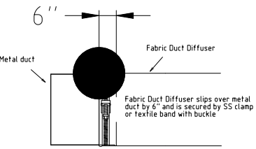
Fabric Duct Inlet connection Detail
