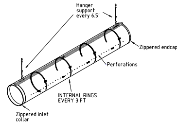
Fabric duct Installation Detail Single Track Profile
